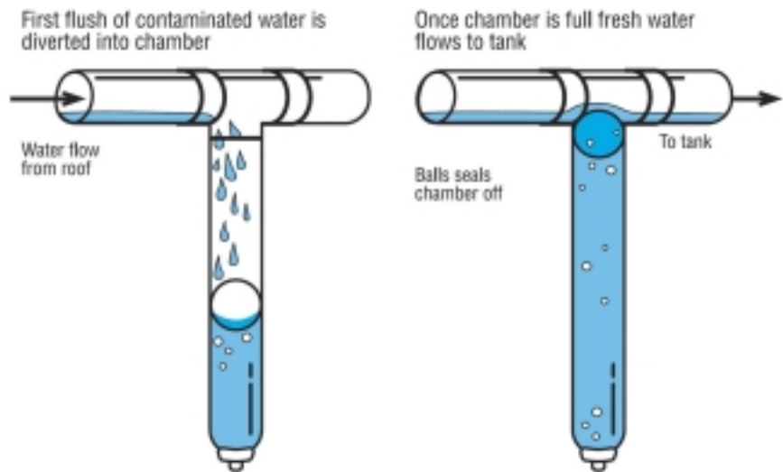
Figure 2. A first flush diverter removes the initial flush of water from the catchment surface so it does not end up in the storage tank. The size of the diverter tube should be proportionate to the catchment surface.
