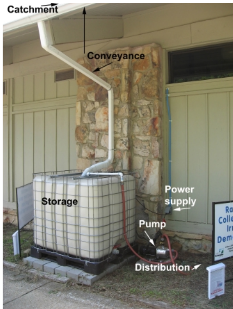
Figure 1. The catchment system is made up of a water catching surface, a conveyance system to get the water to storage, a storage container, and a method of redistribution.
